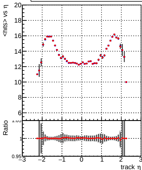
mean hit — DQM_V0001_R000000001_Global_mkFitbase1_RECO — DQM_V0001_R000000001_Global_mkFitbase2_RECO
