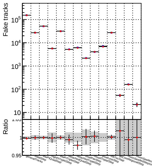
Number —●— DQM_V0001 R000000001 Global mkFitbase2 RECO
