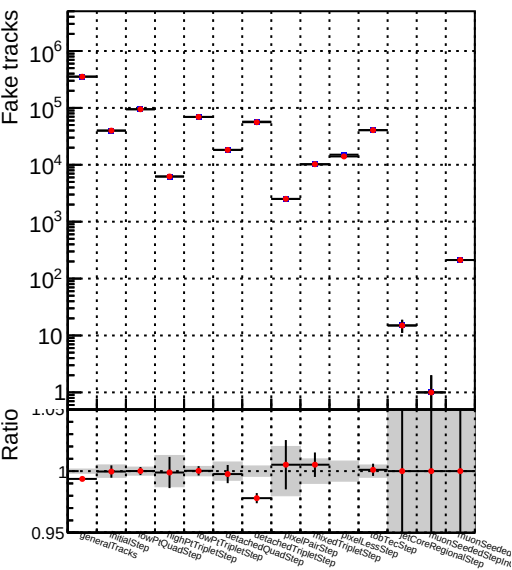
Number ● DQM_V0001_R000000001_Global_mkFitbase2_RECO
