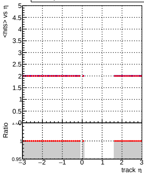
mean hits vs \eta Legend: DQM_V0001_R000000001_Global_mkFitbase1_RECO (blue line), DQM_V0001_R000000001_Global_mkFitbase2_RECO (red line)
