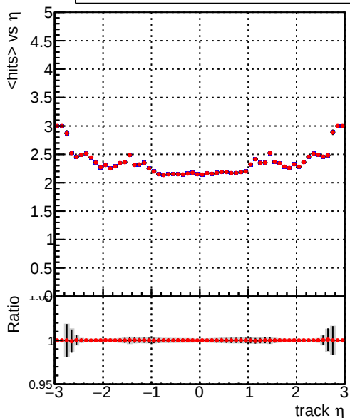
mean hits — DQM_V0001_R000000001_Global_mkFitbase1_RECO — DQM_V0001_R000000001_Global_mkFitbase2_RECO
