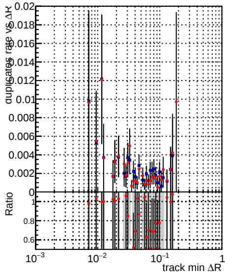
—●— DQM_V0001_R000000001_Global_mkFitbase1_RECO —●— DQM_V0001_R000000001_Global_mkFitbase2_RECO
