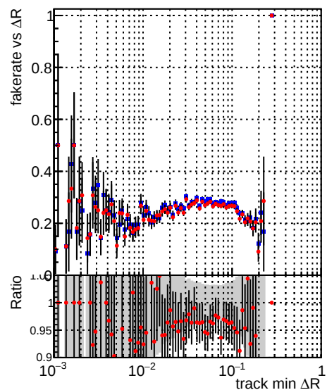
—●— DQM_V0001_R000000001_Global_mkFitbase1_RECO —●— DQM_V0001_R000000001_Global_mkFitbase2_RECO
