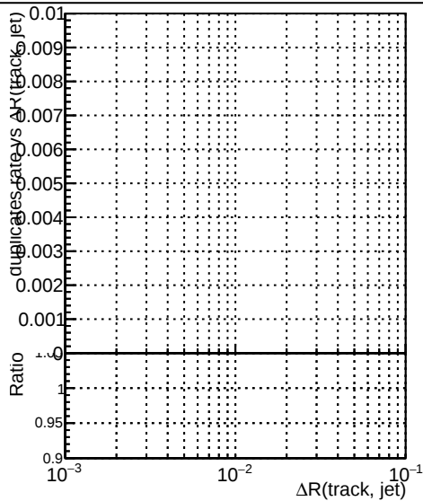
—●— DQM_V0001_R000000001_Global_mkFitbase1_RECO —●— DQM_V0001_R000000001_Global_mkFitbase2_RECO
