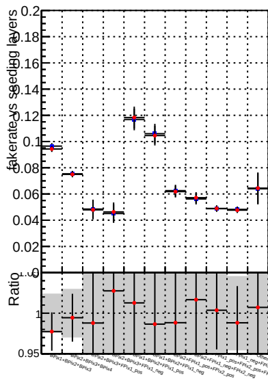
Fake rate vs. Legend Global mkFitbase1 RECO Blue line with circles DQM_V0001_R0000000001 Global mkFitbase1 Red line with circles DQM_V0001_R0000000001 Global mkFitbase2
