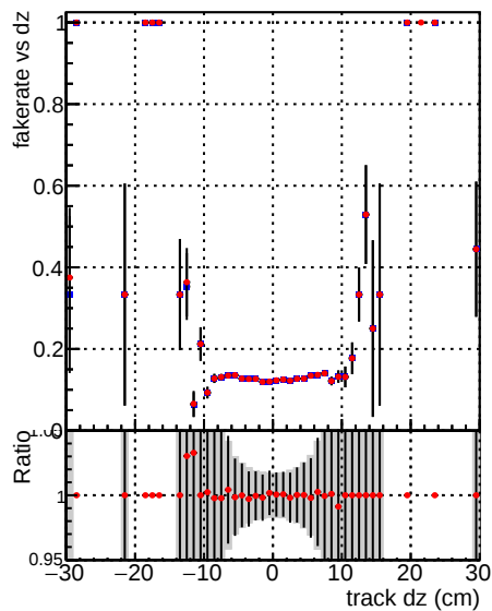
Fake rate vs dz DQM V0001_R000000001 Global mkFitbase1 RECO DQM V0001_R000000001 Global mkFitbase2 RECO
