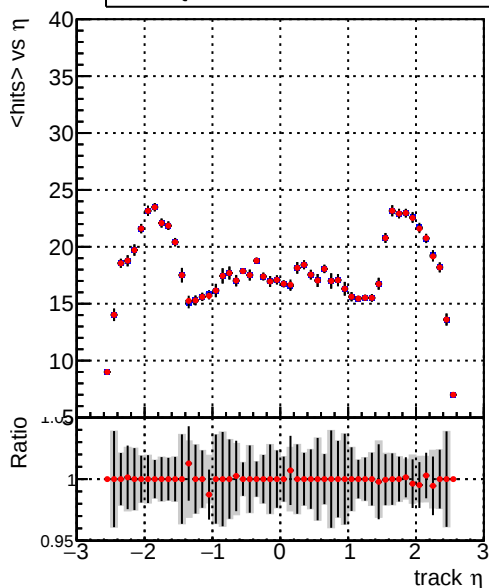
mean hits vs \eta — DQM_V0001_R000000001_Global_mkFitbase1_RECO — DQM_V0001_R000000001_Global_mkFitbase2_RECO
