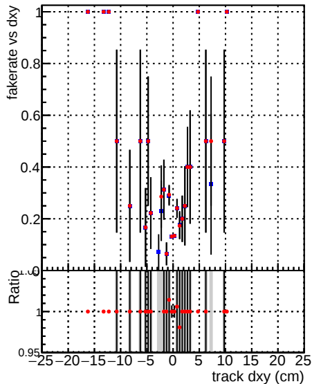
—●— DQM_V0001_R0000000001_Global_mkFitbase1_RECO —●— DQM_V0001_R0000000001_Global_mkFitbase2_RECO
