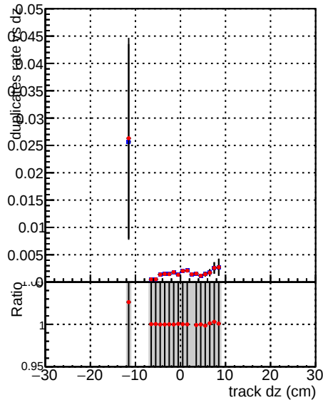
—●— DQM_V0001_R0000000001_Global_mkFitbase1_RECO —●— DQM_V0001_R0000000001_Global_mkFitbase2_RECO
