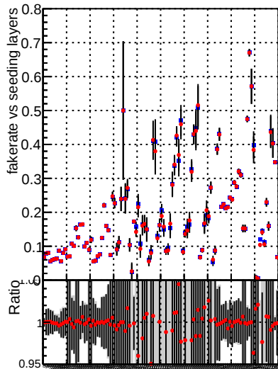
Fake rate vs. —●— DQM V0001_R000000001 Global mkFitbase1 RECO —●— DQM V0001_R000000001 Global mkFitbase2 RECO
