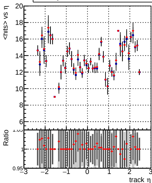
— DQM_V0001_R000000001_Global_mkJFitbase1_RECO — DQM_V0001_R000000001_Global_mkJFitbase2_RECO
