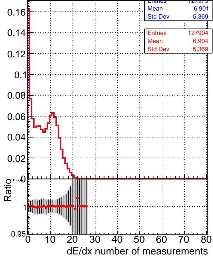
■ DQM_V0001_R000000001_Global_mkFitbase1_RECO ● DQM_V0001_R000000001_Global_mkFitbase2_RECO
