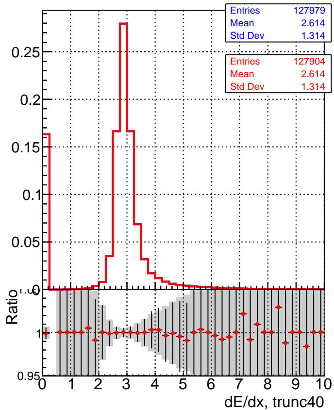
■ DQM_V0001_R000000001_Global_mkFitbase1_RECO ● DQM_V0001_R000000001_Global_mkFitbase2_RECO
