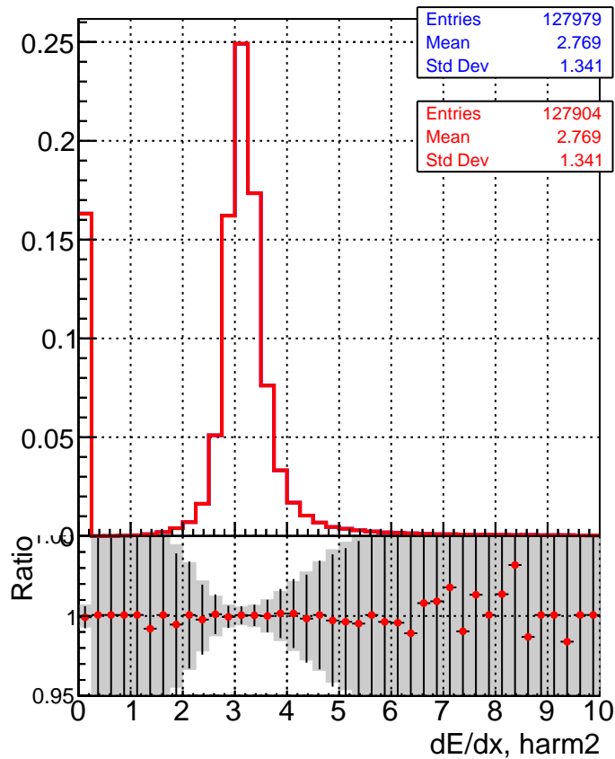
■ DQM_V0001_R000000001_Global_mkFitbase1_RECO ● DQM_V0001_R000000001_Global_mkFitbase2_RECO
