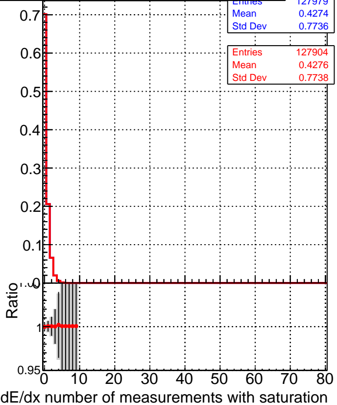
■ DQM_V0001_R000000001_Global_mkFitbase1_RECO ● DQM_V0001_R000000001_Global_mkFitbase2_RECO
