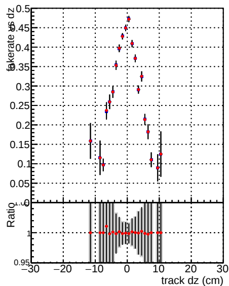
—●— DQM_V0001_R0000000001_Global_mkFitbase1_RECO —●— DQM_V0001_R0000000001_Global_mkFitbase2_RECO
