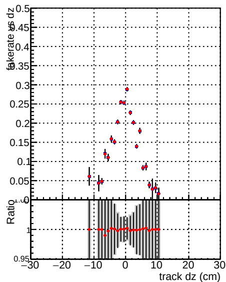
DQM V0001_R0000000001 Global mkFitbase1 RECO Fake rate vs d Duplicates Rate vs Dxy Pileup rate vs dxy
