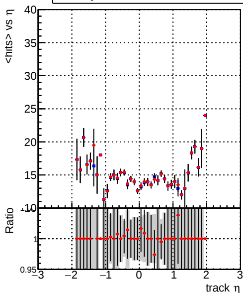
mean hits vs \eta Legend: DQM_V0001_R000000001_Global_mkFitbase1_RECO (blue line with markers), DQM_V0001_R000000001_Global_mkFitbase2_RECO (red line with markers)
