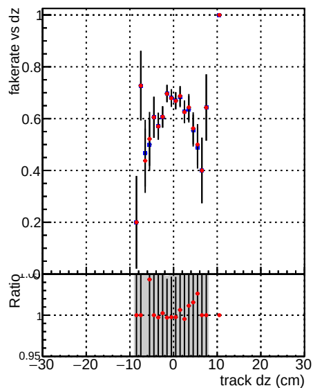
Fake rate vs d DQM V0001_R0000000001 Global mkFitbase1 RECO DQM V0001_R0000000001 Global mkFitbase2 RECO
