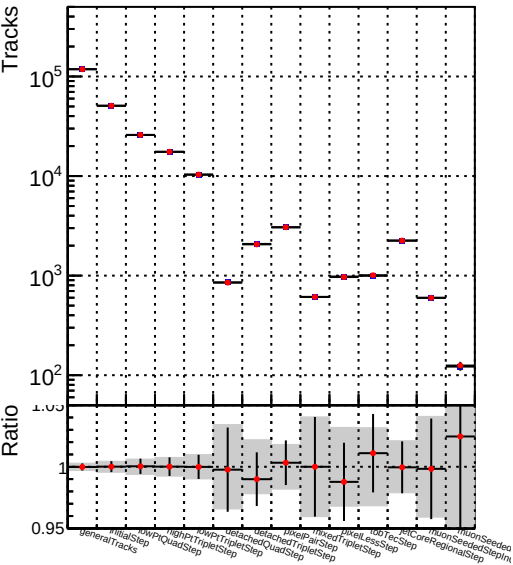
■ DQM_V0001_R000000001_Global_mkFitbase1_RECO
