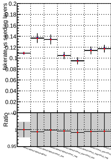
Fake rate vs. Legend DQM V0001_R000000001 Global mkFitbase1 RECO Blue line with dots Red line with dots
