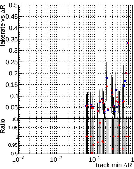
Fake rate vs \Delta R(\text{track}, \text{jet}) Legend: DQM_V0001_R000000001_Global_mkFitbase1_RECO DQM_V0001_R000000001_Global_mkFitbase2_RECO
