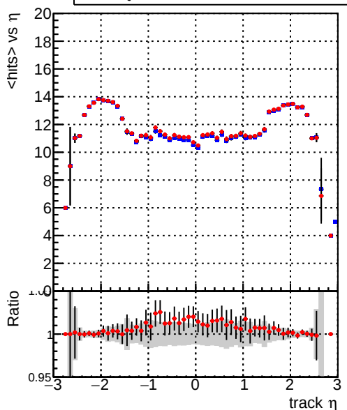
mean hits vs \eta Legend: DQM_V0001_R000000001_Global_mkFitbase1_RECO (blue), DQM_V0001_R000000001_Global_mkFitbase2_RECO (red)
