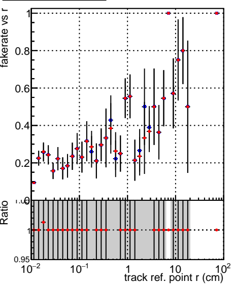
■ DQM_V0001_R000000001_Global_mkFitbase1_RECO ● DQM_V0001_R000000001_Global_mkFitbase2_RECO
