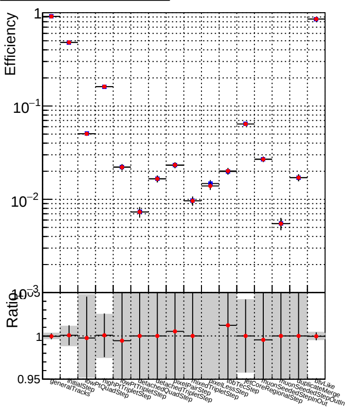
DQM_V0001_R000000001_Global_mkFitbase1_RECO DQM_V0001_R000000001_Global_mkFitbase2_RECO
