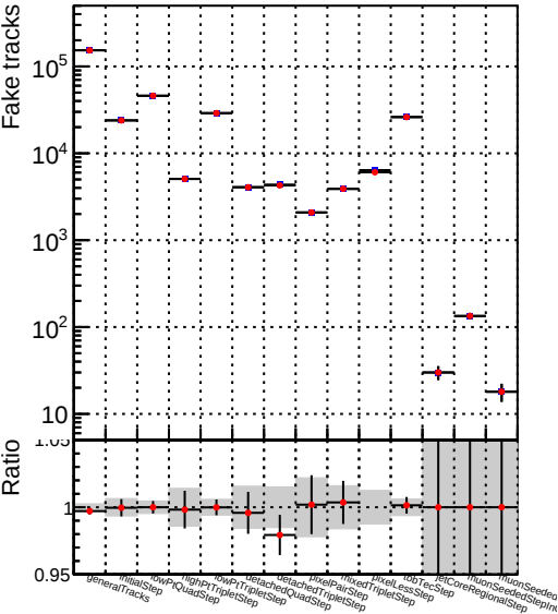
Number ● DQM_V0001_R000000001_Global_mkFitbase2_RECO
