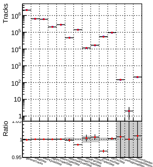
DQM_V0001_R000000001_Global_mkFitbase1_RECO
