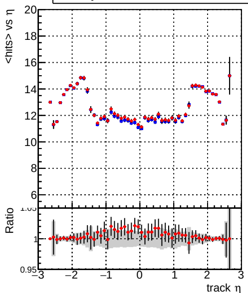
— DQM_V0001_R000000001_Global_mkFitbase1_RECO — DQM_V0001_R000000001_Global_mkFitbase2_RECO
