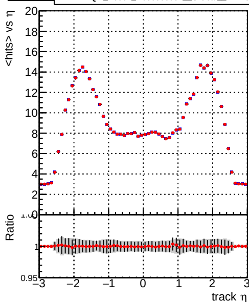
— DQM_V0001_R000000001_Global_mkFitbase1_RECO — DQM_V0001_R000000001_Global_mkFitbase2_RECO
