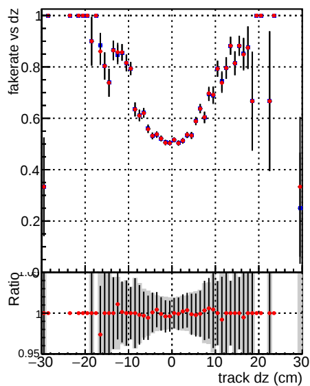
Fake rate vs dz Global mkFitbase1 RECO DQM V0001_R000000001 Global mkFitbase2 RECO
