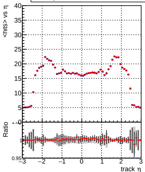
— DQM_V0001_R000000001_Global_mkJFitbase1_RECO — DQM_V0001_R000000001_Global_mkJFitbase2_RECO
