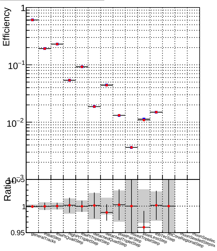
DQM_V0001_R000000001_Global_mkFitbase1_RECO DQM_V0001_R000000001_Global_mkFitbase2_RECO
