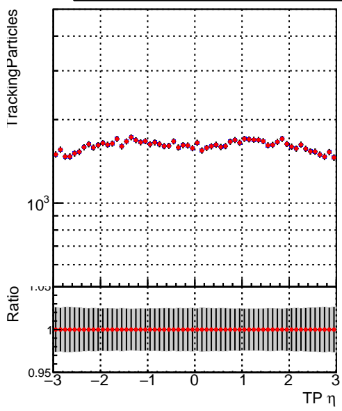
N of simulated tracks vs \eta Legend: - \square DQM_V0001_R000000001_Global_mkFitbase1_RECO - \bullet DQM_V0001_R000000001_Global_mkFitbase2_RECO
