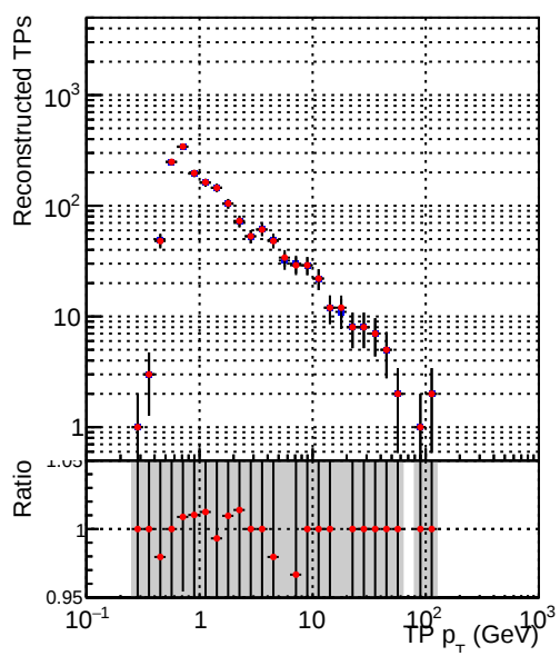
— DQM_V0001_R000000001_Global_mkFitbase1_RECO — DQM_V0001_R000000001_Global_mkFitbase2_RECO
