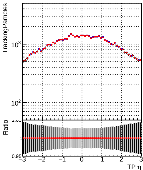
— DQM_V0001_R000000001_Global_mkFitbase1_RECO — DQM_V0001_R000000001_Global_mkFitbase2_RECO
