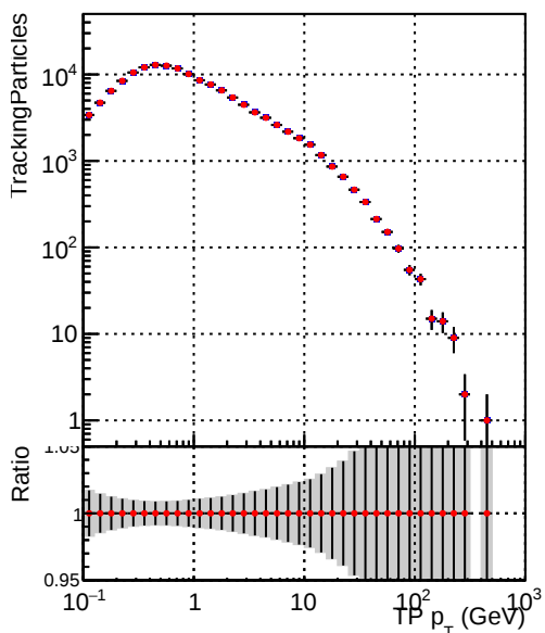
— DQM_V0001_R000000001_Global_mkFitbase1_RECO — DQM_V0001_R000000001_Global_mkFitbase2_RECO
