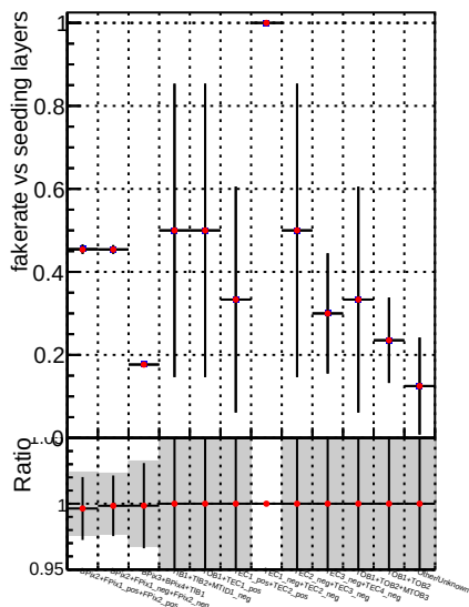
Fake rate vs. —●— DQM V0001_R000000001 Global mkFitbase1 RECO —●— DQM V0001_R000000001 Global mkFitbase2 RECO
