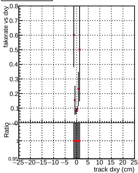
Global mkFitbase1 RECO Fake rate vs d DQM V0001_R000000001 DQM V0001_R000000001 DQM V0001_R000000001 Duplicates Rate vs Dxy DQM V0001_R000000001 DQM V0001_R000000001 DQM V0001_R000000001 Pileup rate vs dxy DQM V0001_R000000001 DQM V0001_R000000001 DQM V0001_R000000001
