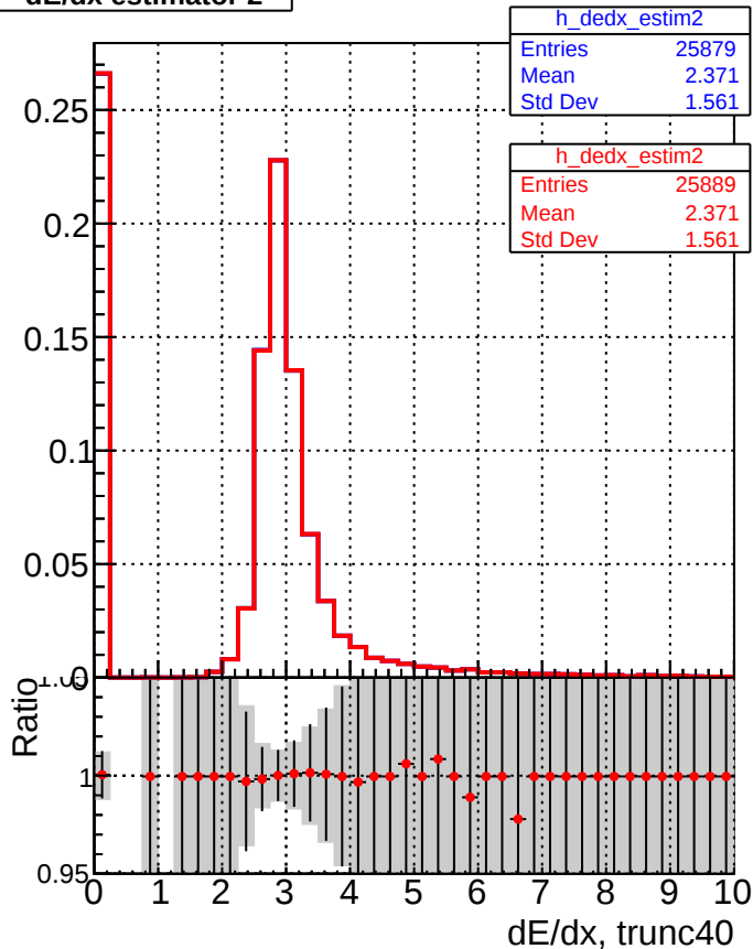
DQM_V0001_R000000001_Global_mkFitbase1_RECO DQM_V0001_R000000001_Global_mkFitbase2_RECO
