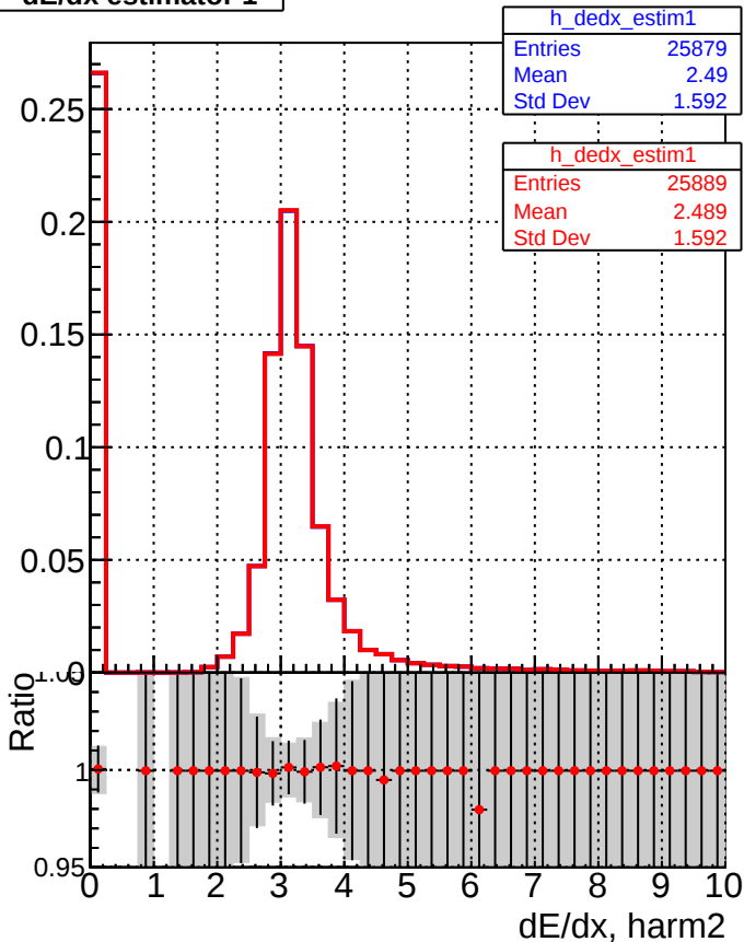
DQM_V0001_R000000001_Global_mkFitbase1_RECO DQM_V0001_R000000001_Global_mkFitbase2_RECO
