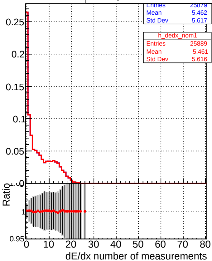
DQM_V0001_R000000001_Global_mkFitbase1_RECO DQM_V0001_R000000001_Global_mkFitbase2_RECO
