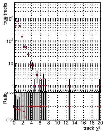
Legend: DQM_V0001_R0000000001_Global_mkFitbase1_RECO DQM_V0001_R0000000001_Global_mkFitbase2_RECO
