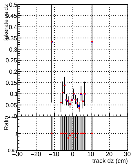
Fake rate vs dz DQM_V0001_R0000000001 Global mkFitbase1 RECO
