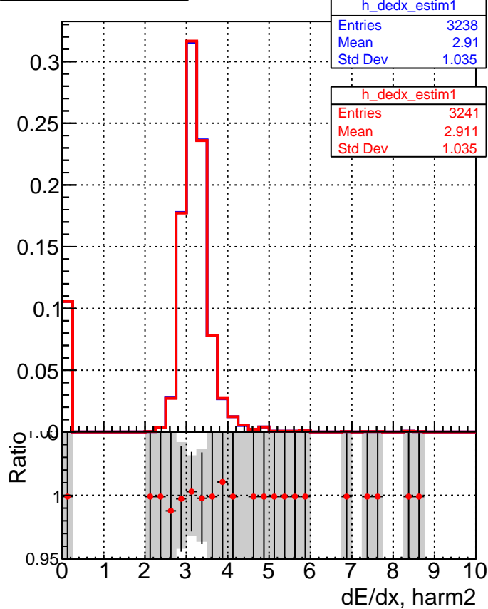
■ DQM_V0001_R000000001_Global_mkFitbase1_RECO ● DQM_V0001_R000000001_Global_mkFitbase2_RECO
