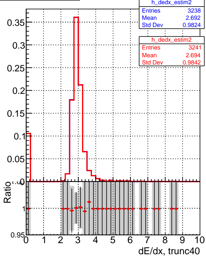
■ DQM_V0001_R000000001_Global_mkFitbase1_RECO ● DQM_V0001_R000000001_Global_mkFitbase2_RECO
