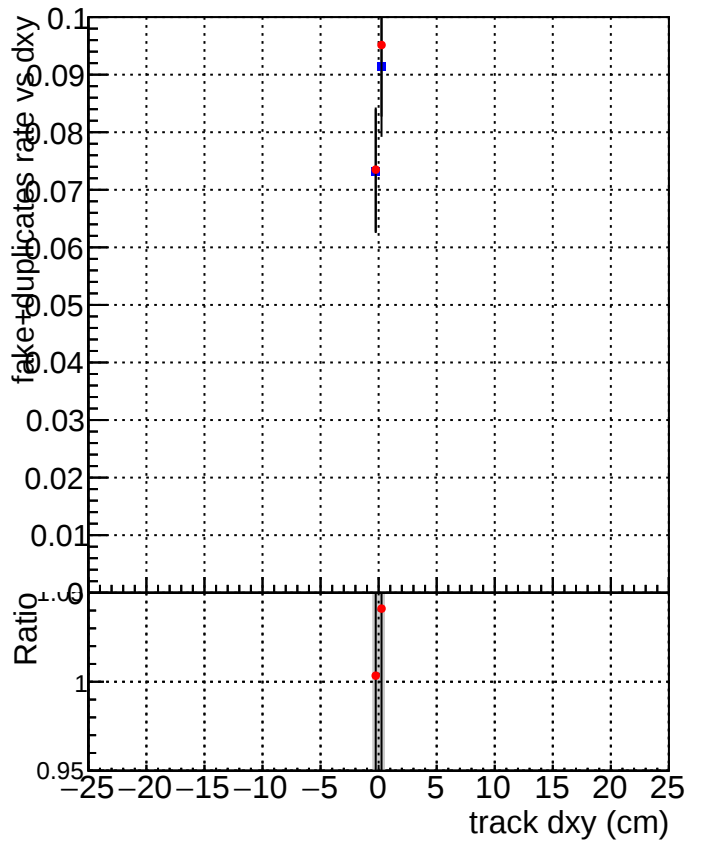
DQM_V0001_R000000001_Global_mkFitbase1_RECO DQM_V0001_R000000001_Global_mkFitbase2_RECO
