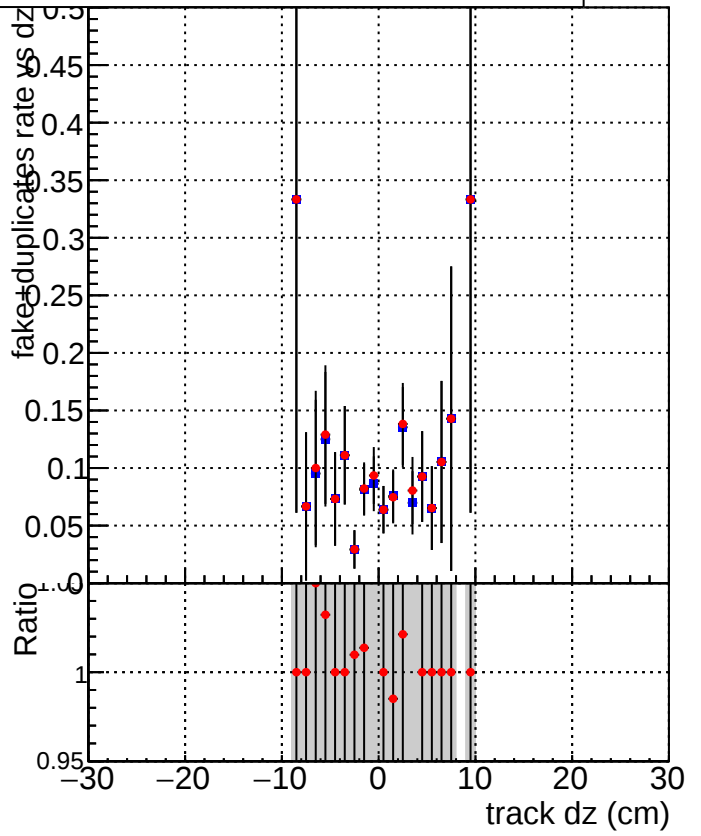
DQM_V0001_R000000001_Global_mkFitbase1_RECO DQM_V0001_R000000001_Global_mkFitbase2_RECO
