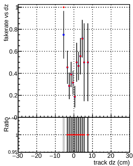
Fake rate vs dz DQM V0001_R000000001 Global mkFitbase1 RECO
