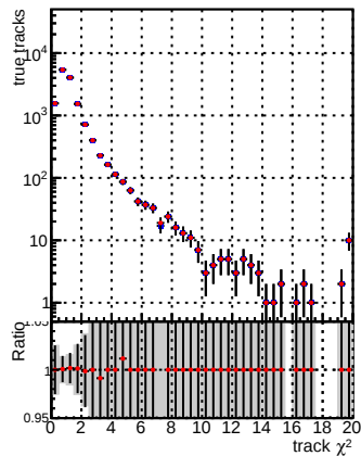
1 Global mkFitbase1 RECO 1 Global mkFitbase2 RECO
