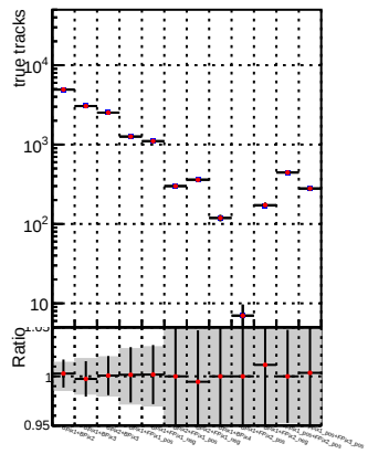
1 Global mkFitbase1 RECO 1 Global mkFitbase2 RECO
