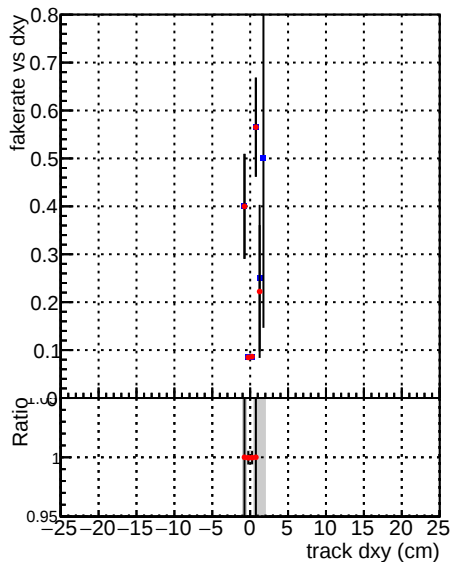
Fake rate vs d DQM_V0001_R0000000001_Global_mkFitbase1_RECO DQM_V0001_R0000000001_Global_mkFitbase2_RECO
