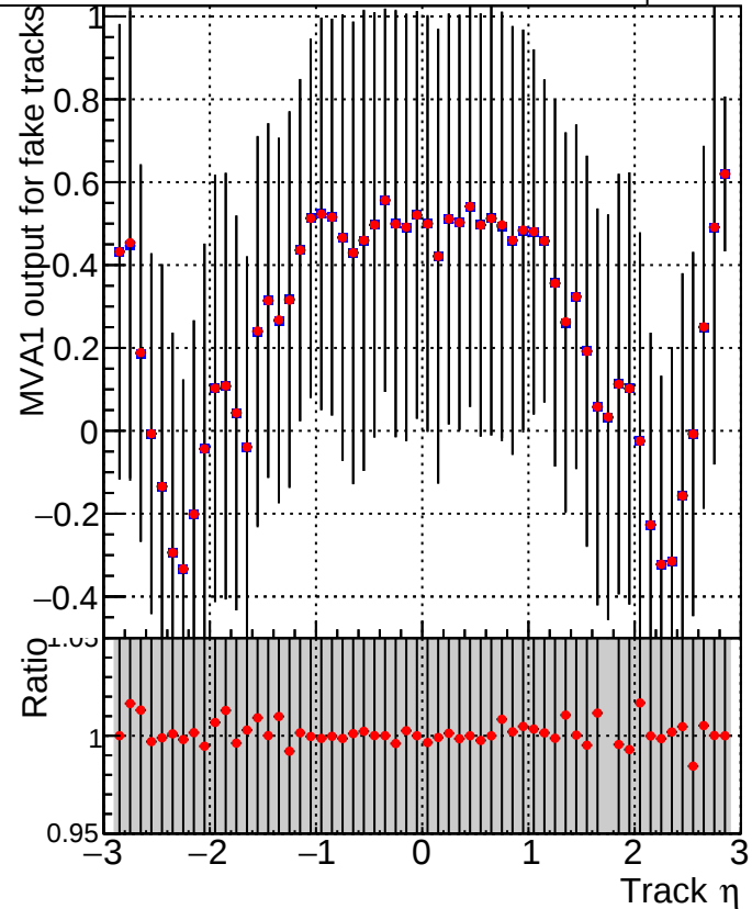
MVA1 of associated tracks (recoToSim) vs. track \eta ■ DQM_V0001_R000000001_Global_mkFitbase1_RECO ● DQM_V0001_R000000001_Global_mkFitbase2_RECO
