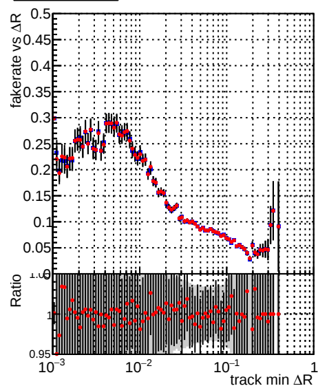
—●— DQM_V0001_R000000001_Global_mkFitbase1_RECO —●— DQM_V0001_R000000001_Global_mkFitbase2_RECO
