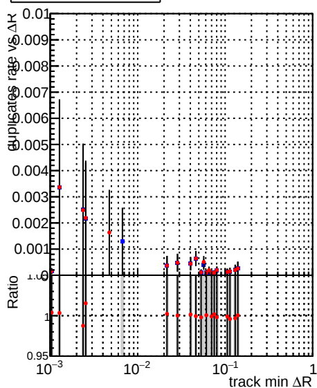
—●— DQM_V0001_R000000001_Global_mkFitbase1_RECO —●— DQM_V0001_R000000001_Global_mkFitbase2_RECO
