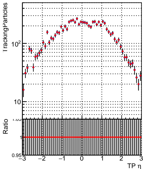
— DQM_V0001_R0000000001_Global_mkFitbase1_RECO — DQM_V0001_R0000000001_Global_mkFitbase2_RECO
