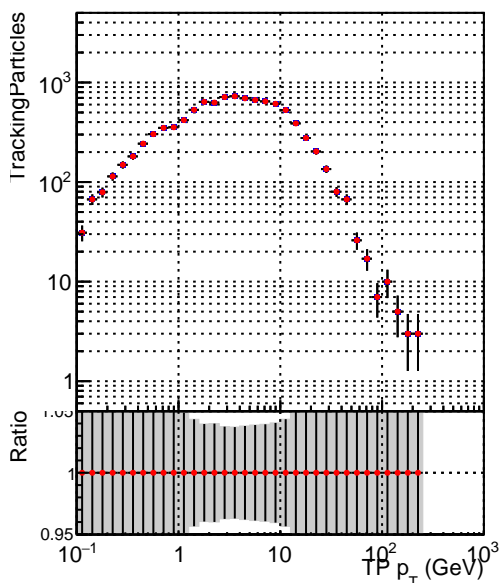
— DQM_V0001_R0000000001_Global_mkFitbase1_RECO — DQM_V0001_R0000000001_Global_mkFitbase2_RECO
