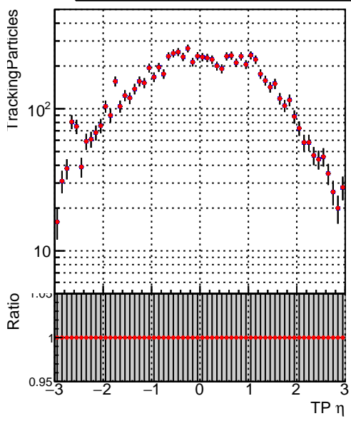
N of simulated tracks vs \eta Legend: DQM_V0001_R0000000001_Global_mkFitbase1_RECO (blue line), DQM_V0001_R0000000001_Global_mkFitbase2_RECO (red line)
