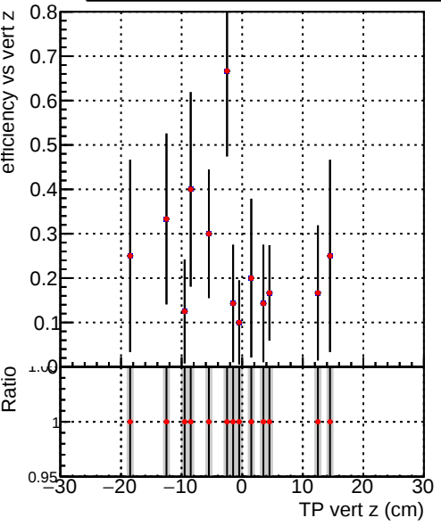
Efficiency vs vert z Legend: DQM_V0001_R000000001_Global_mkFit10muon-base1_RECO DQM_V0001_R000000001_Global_mkFit10muon-base2_RECO
