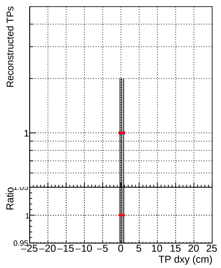
N of simulated track DQM_V0001_R000000001_Global_mkFit10muon-base1_RECO DQM_V0001_R000000001_Global_mkFit10muon-base2_RECO
