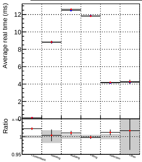
Average DQM_V0001_R000000001_Global_mkFit10muon-base1_RECO DQM_V0001_R000000001_Global_mkFit10muon-base2_RECO
